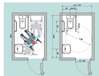
Fig. V.43. Amenajarea unei cabine WC adaptate - tip B
