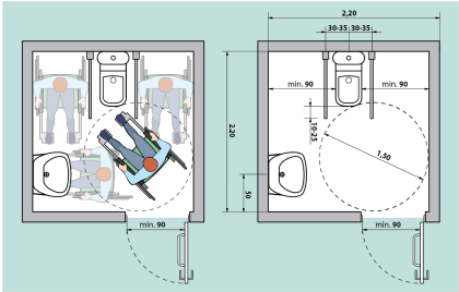
Fig. V.42a Aranjarea unei cabine WC adaptate - tip A
