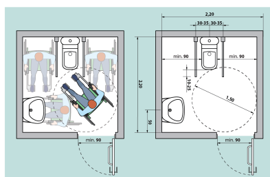
Fig. V.42.1 Amenajarea unei cabine WC adaptate - tip A
