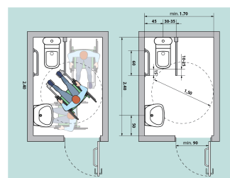
Fig. V.41.a Aranjarea unei cabine WC adaptate - tip B
